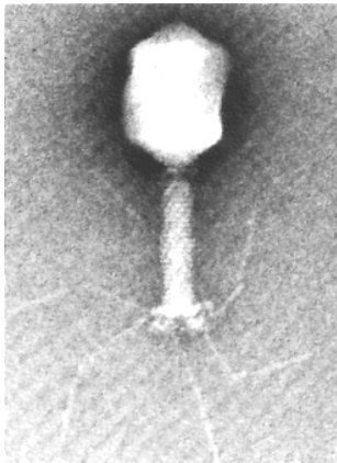
Viral Structure
